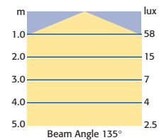
Data for 26 watt c/w Opal Cover
