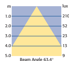
Data for 26 watt c/w Prismatic Cover
