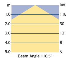
Data for 26 watt c/w Halo Ring
